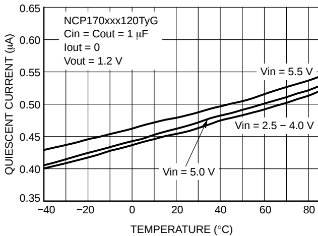
Figure 15. Quiescent Current vs. Temperature, V_{out} = 1.2\text{ V}
